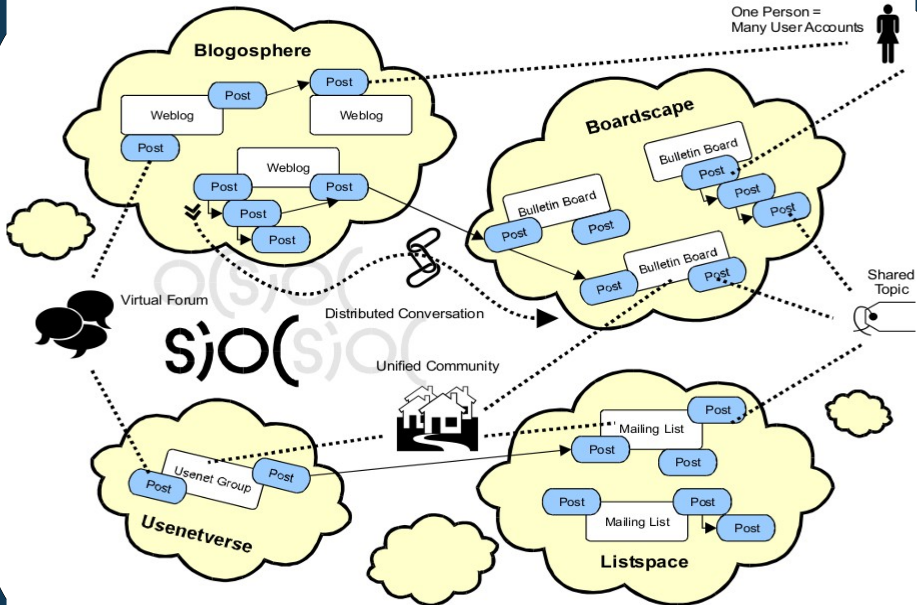
Creating connections between discussion clouds with SIOC
